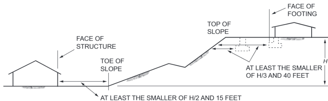
FIGURE R403.1.9.1 FOUNDATION CLEARANCE FROM SLOPES
